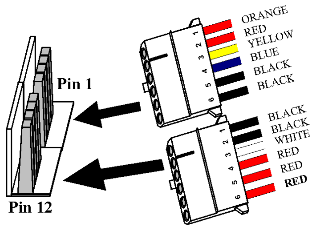
Power Supply Connector
